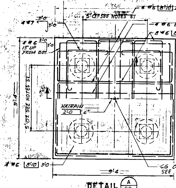
PLAN - SUGGESTED PILE CAP
