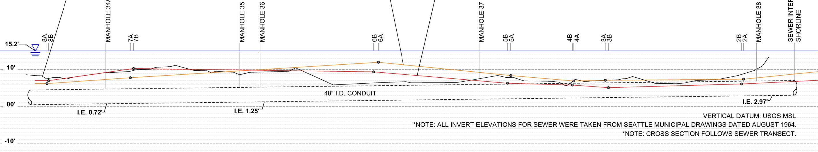
FIGURE 3 PROFILE SECTION ALONG SEWER TRANSECT
