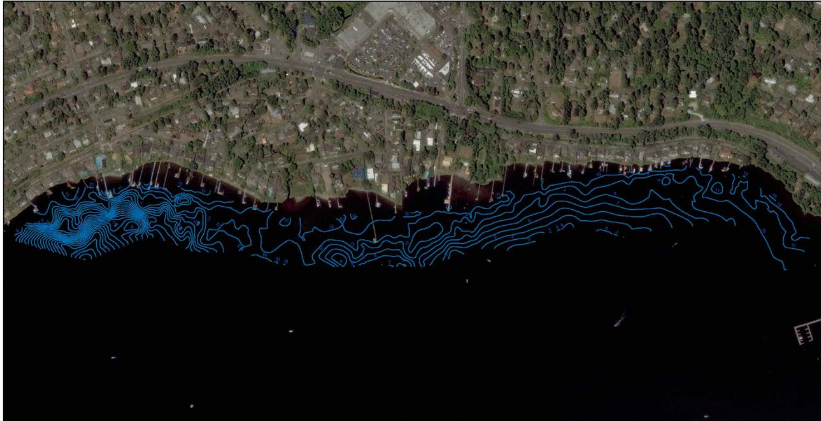
Figure 3. Bathymetric contours at 1-foot intervals
