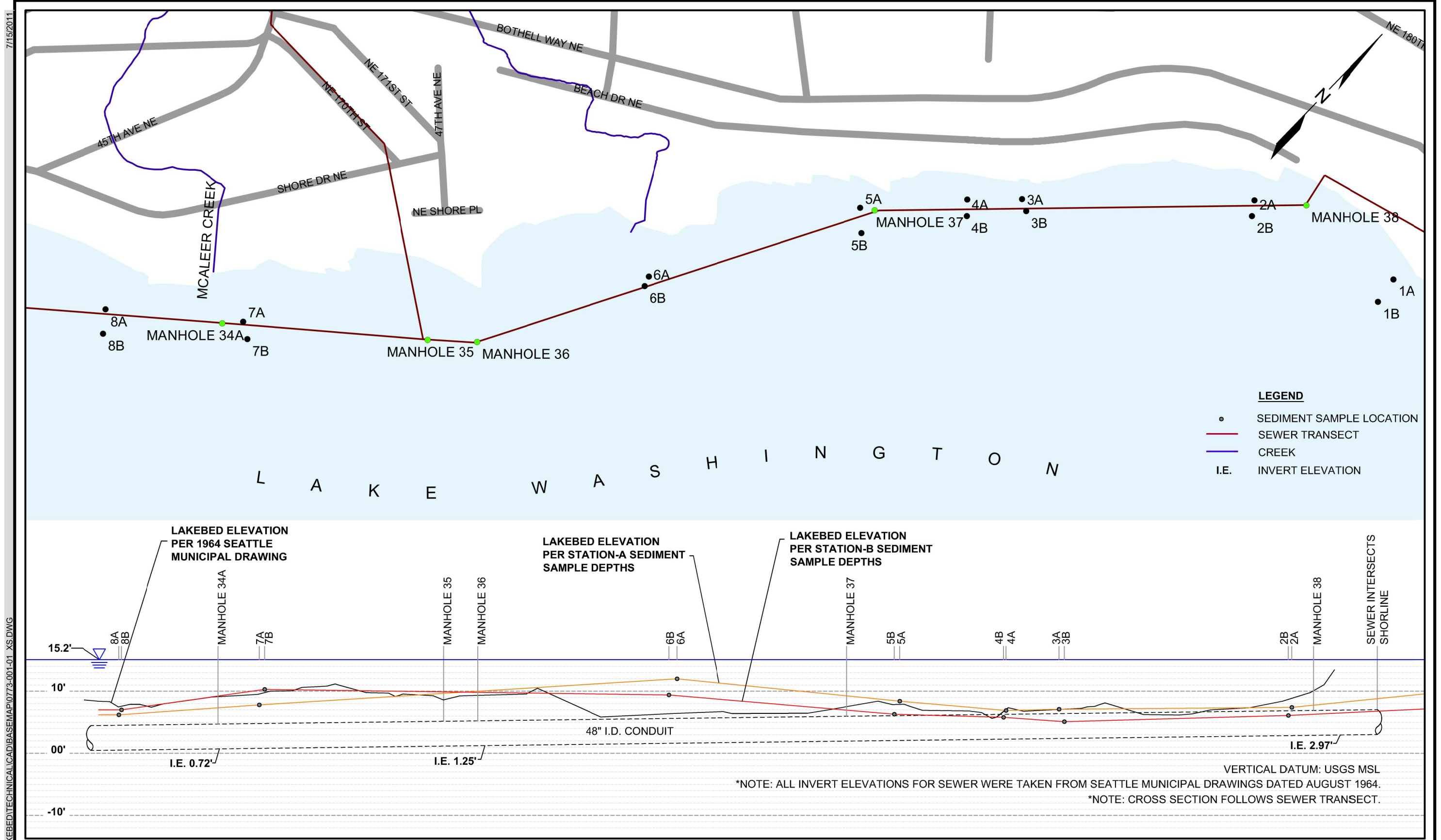
FIGURE 3 PROFILE SECTION ALONG SEWER TRANSECT
