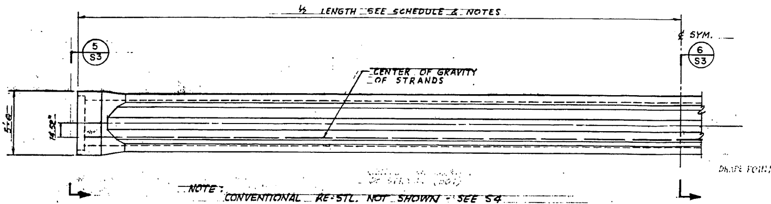
ELEVATION PRESTRESSED PIPE BEAM - DETAIL NO SCALE
